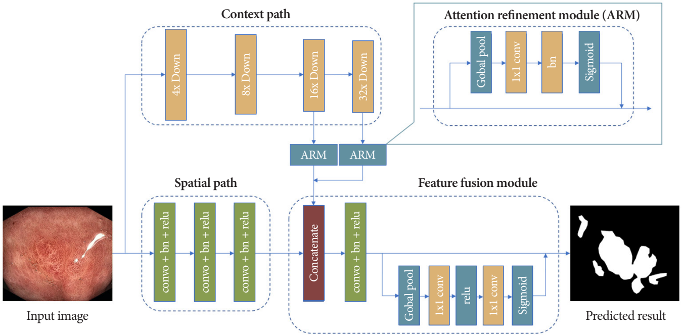
Supplementary Fig. 4. Model architecture of the bilateral segmentation network (BiSeNet). There are two main paths and two modules.
