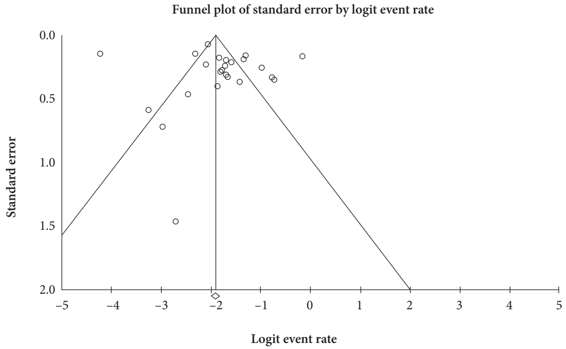
Supplementary Fig. 1. Funnel plot for publication bias in studies assessing post-ERCP complications in cirrhosis.
